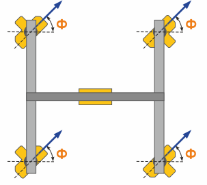
Diagonal movement (crab)
