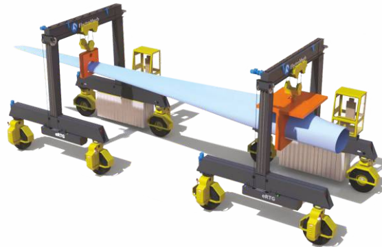
Windmill blade
